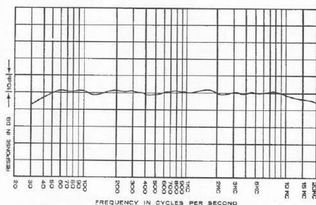
Figure 1 - Frequency Response
